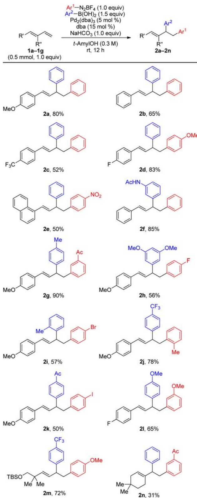
Figure 1. Exploration of the scope of coupling partners in the three-component diarylation of terminal 1,3-butadienes. The isolated yield of each product is reported.
