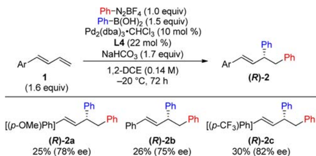
Figure 2. Reoptimized enantioselective diphenylations of ( E )-1-aryl-1,3-dienes at -20\text{ }^{\circ}\text{C} . The isolated yield and enantiomeric excess (as determined by SFC) for each product are reported.
